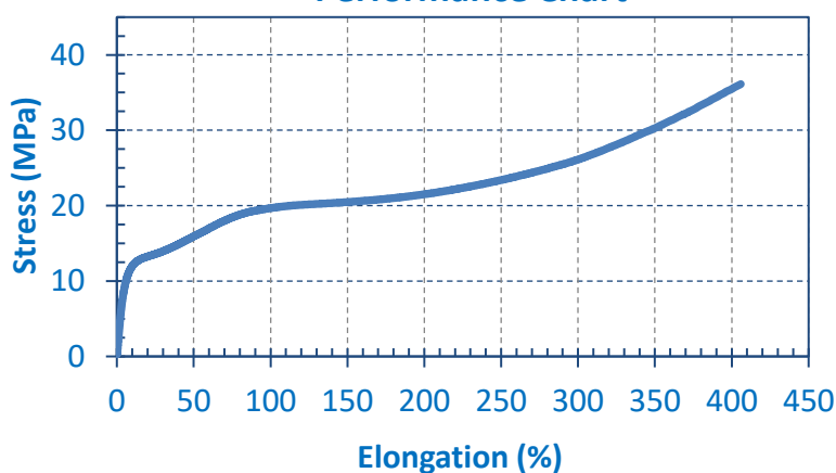
Fiber Film Alpha-HD Performance Chart
