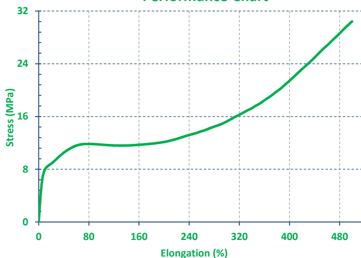
Eco Fiber Film Performance Chart
